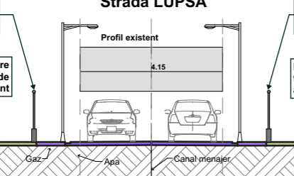
Sectiune transversala 1-1 (sc 1:100)
