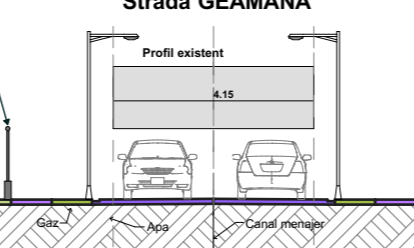
Sectiune transversala 2-2 (sc 1:100)
